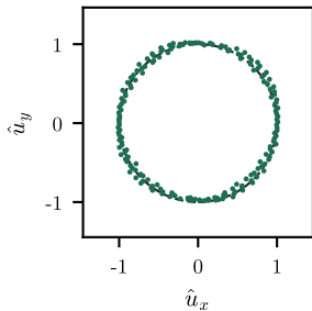
(b) 回拉单位圆 \kappa(\hat{\mathbf{A}}) = 45.24
