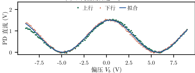
(a) 双向直流传递 V_\pi = 5.278 V
