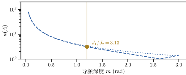
(c) \kappa(A) 理论曲线
