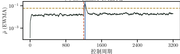
(b) 圆残差监测与阈值 \rho_{th} = 0.06
