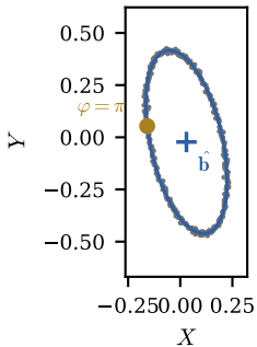
(a) raw observable plane
