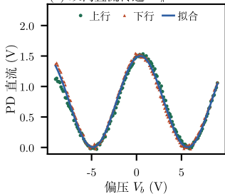
(a) 双向直流传递 V_\pi = 5.278 V
