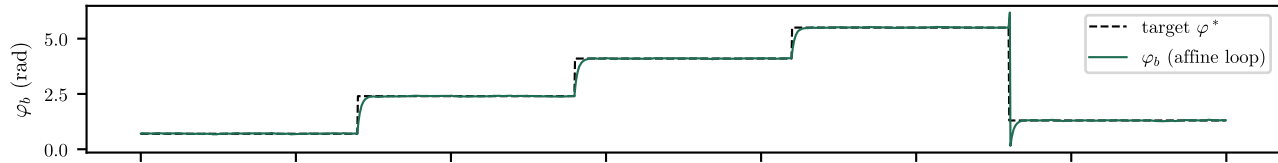
(a) MZM setpoint staircase across arbitrary points
