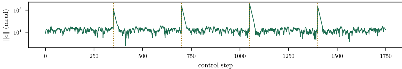
(b) DPMZM: three-axis setpoint steps (dotted: step instants)
