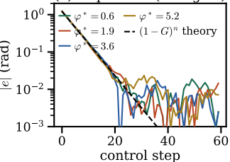
(a) acquisition (4 targets)
