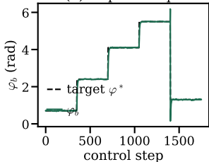
(b) setpoint steps
