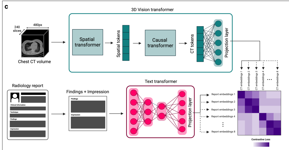
Figure 2.8: CT-CLIP architecture
