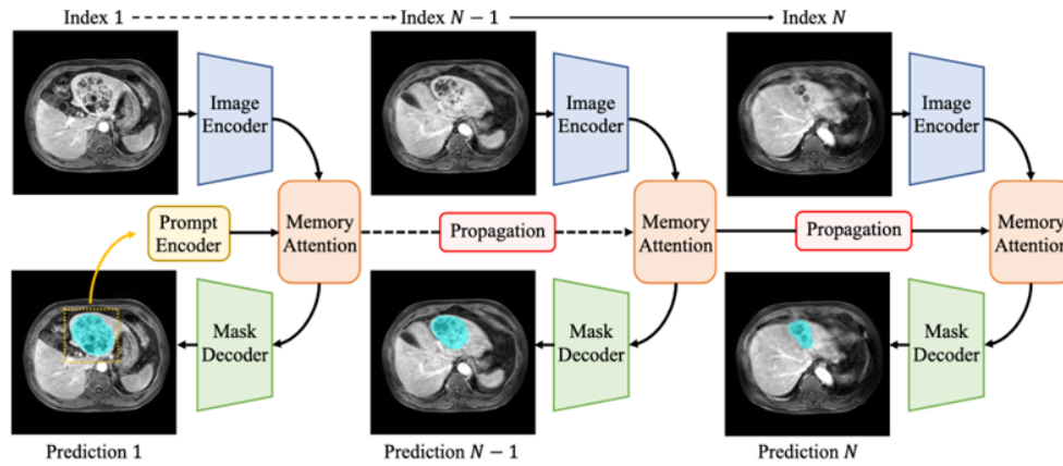
Figure 2.7: Architecture of MedSAM2
