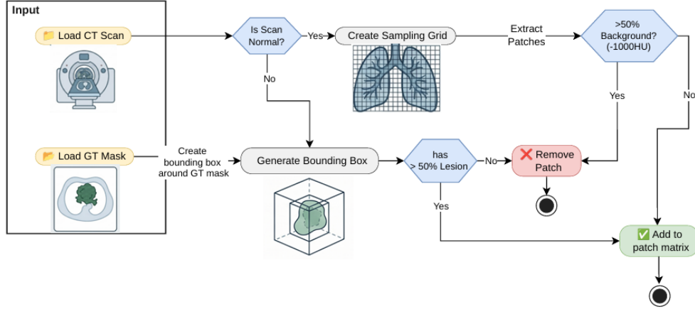
Figure 3.7: Patch extraction workflow.
