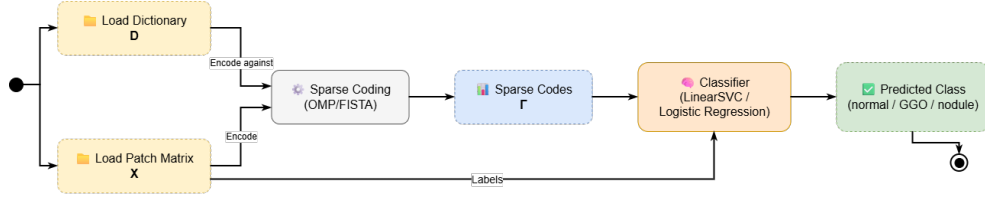
Figure 3.3: Overview of the classification pipeline: each patch is first converted into a sparse code \Gamma against the frozen dictionary D (Section 3.2.1), and the resulting codes are then used to train and query a classifier that predicts the patch-level class label (Section 3.2.2).
