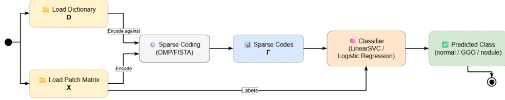
Figure 3.5: Overview of the classification pipeline: each patch is first converted into a sparse code \Gamma against the frozen dictionary D (Section 3.2.1), and the resulting codes are then used to train and query a classifier that predicts the patch-level class label (Section 3.2.2).
