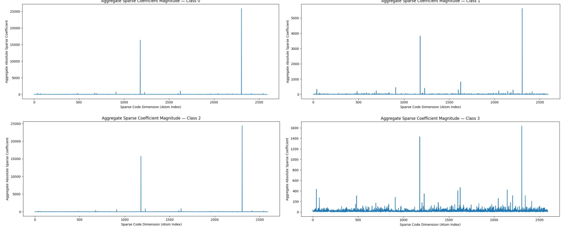
Figure 3.10: Mean absolute sparse coefficients for each atom across all classes in the LC-KSVD dictionary.
