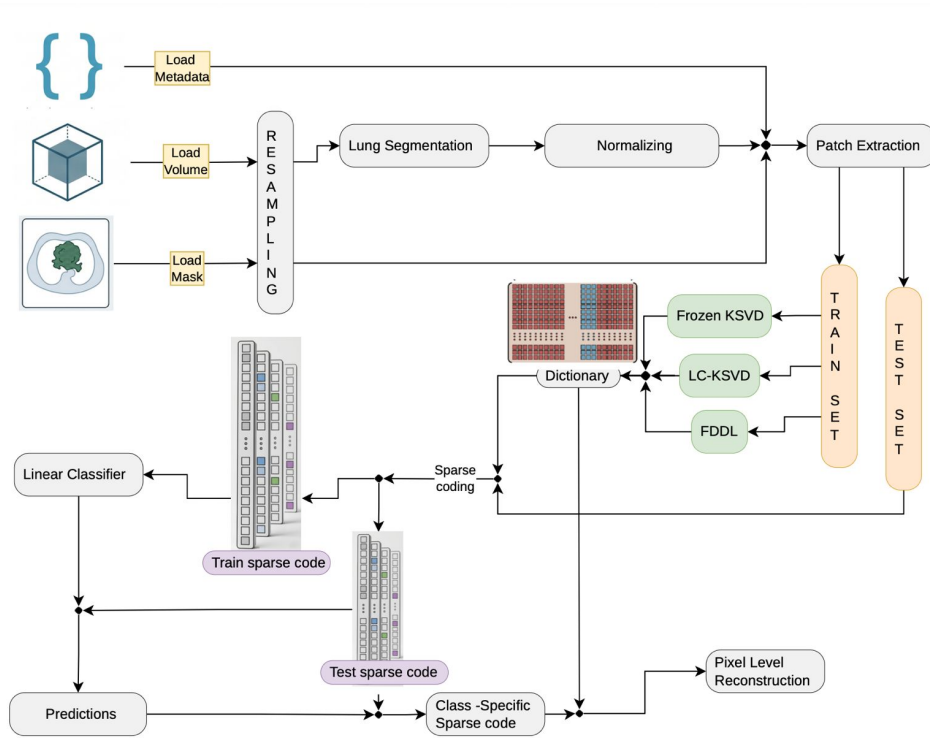
Figure 3.1: Overall Methodology Diagram.
