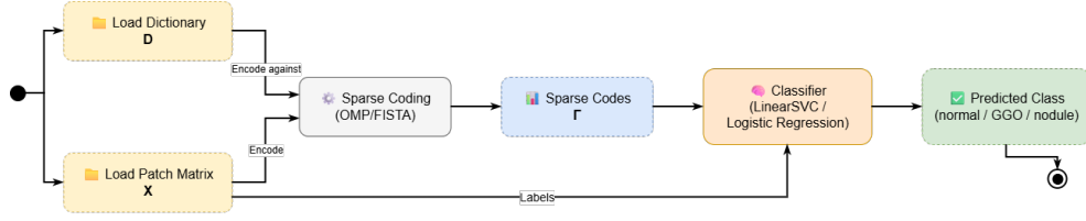
Figure 3.9: Overview of the classification pipeline: each patch is first converted into a sparse code \Gamma against the frozen dictionary D (Section 3.2.1), and the resulting codes are then used to train and query a classifier that predicts the patch-level class label (Section 3.2.2).
