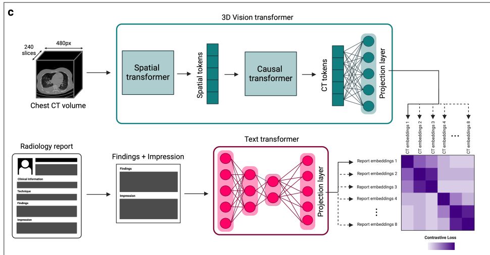
Figure 2.6: CT-CLIP architecture
