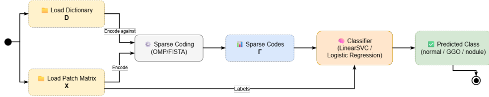
Figure 3.8: Overview of the classification pipeline: each patch is first converted into a sparse code \Gamma against the frozen dictionary D (Section 3.2.1), and the resulting codes are then used to train and query a classifier that predicts the patch-level class label (Section 3.2.2).
