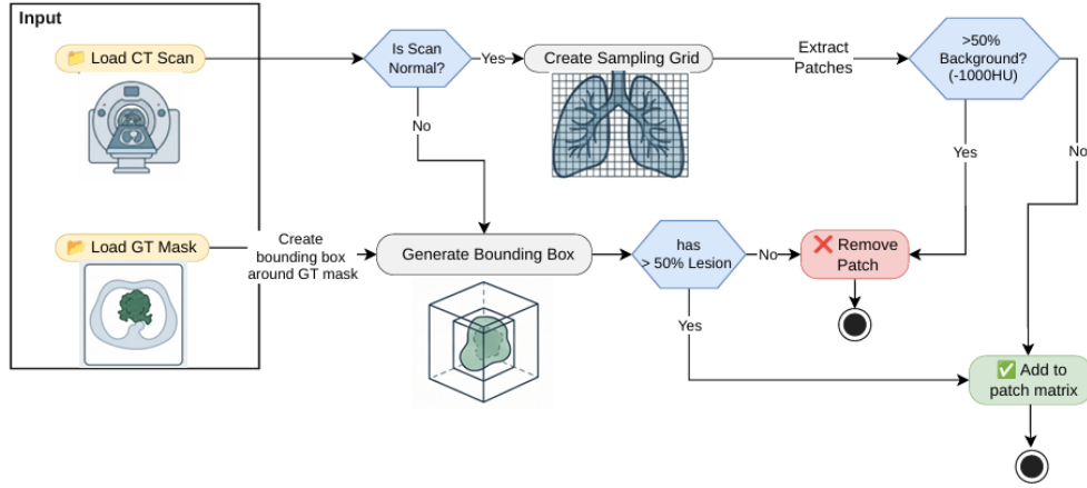
Figure 3.7: Patch extraction workflow, showing the normal-scan sampling grid and the lesion bounding-box branch for annotated scans, each filtered by its own background/lesion-fraction threshold before patches are added to the patch matrix.
