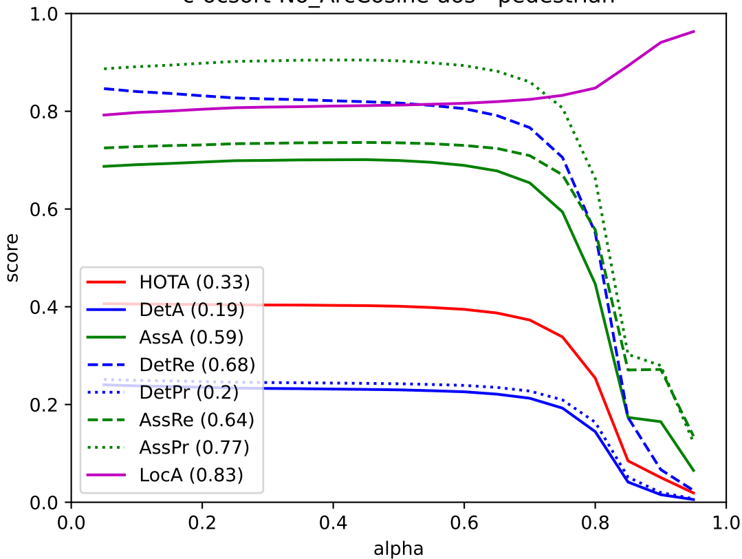
c-ocsort-No_ArcCosine-aos - pedestrian
