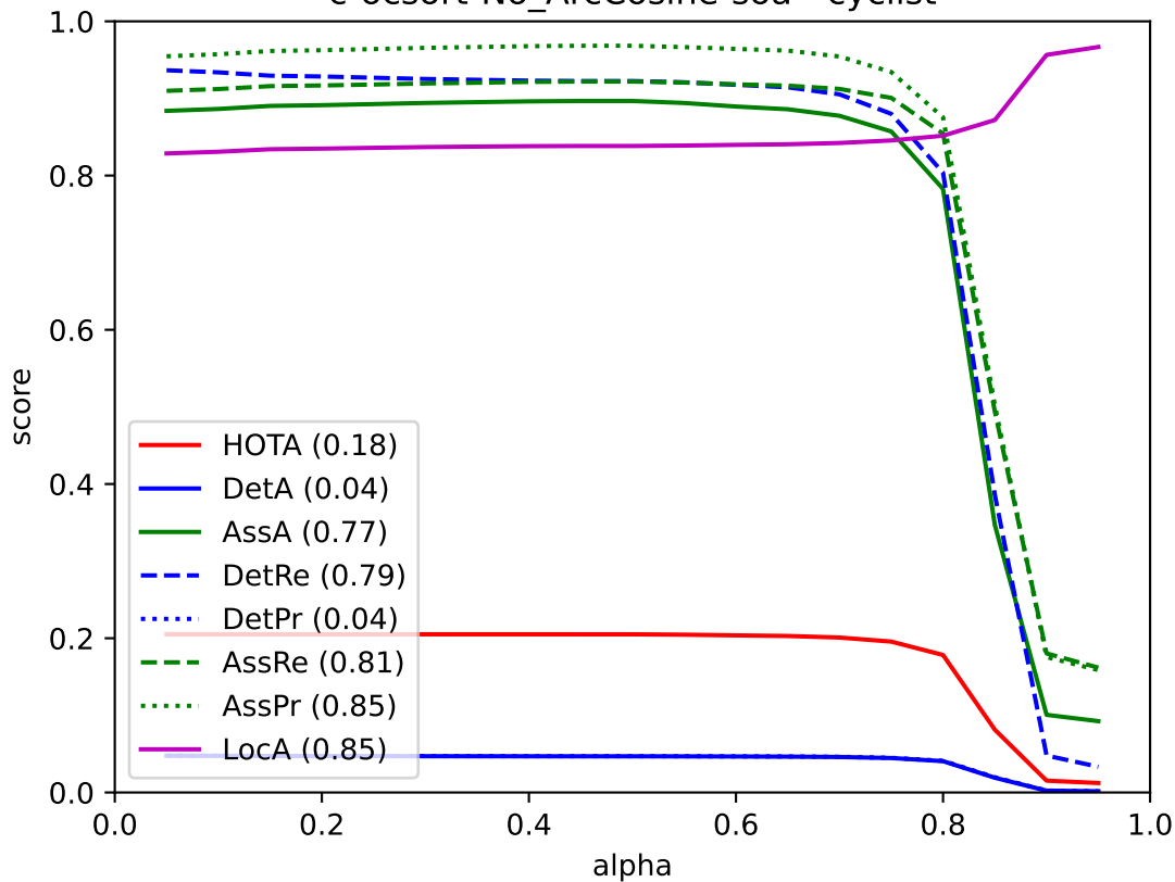
c-ocsort-No_ArcCosine-soa - cyclist
