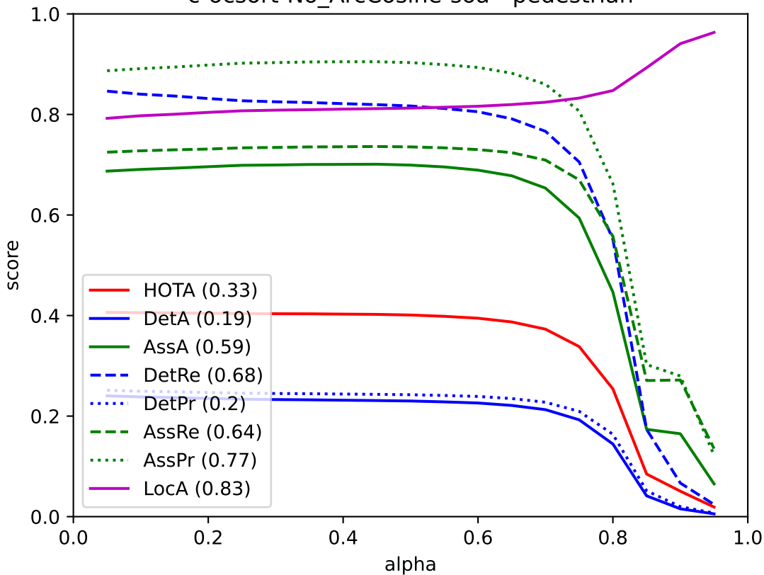
c-ocsort-No_ArcCosine-soa - pedestrian
