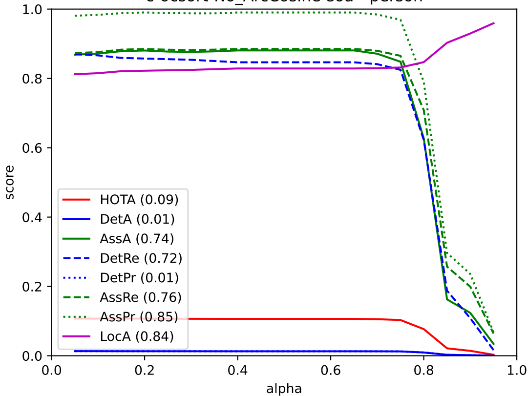
c-ocsort-No_ArcCosine-soa - person
