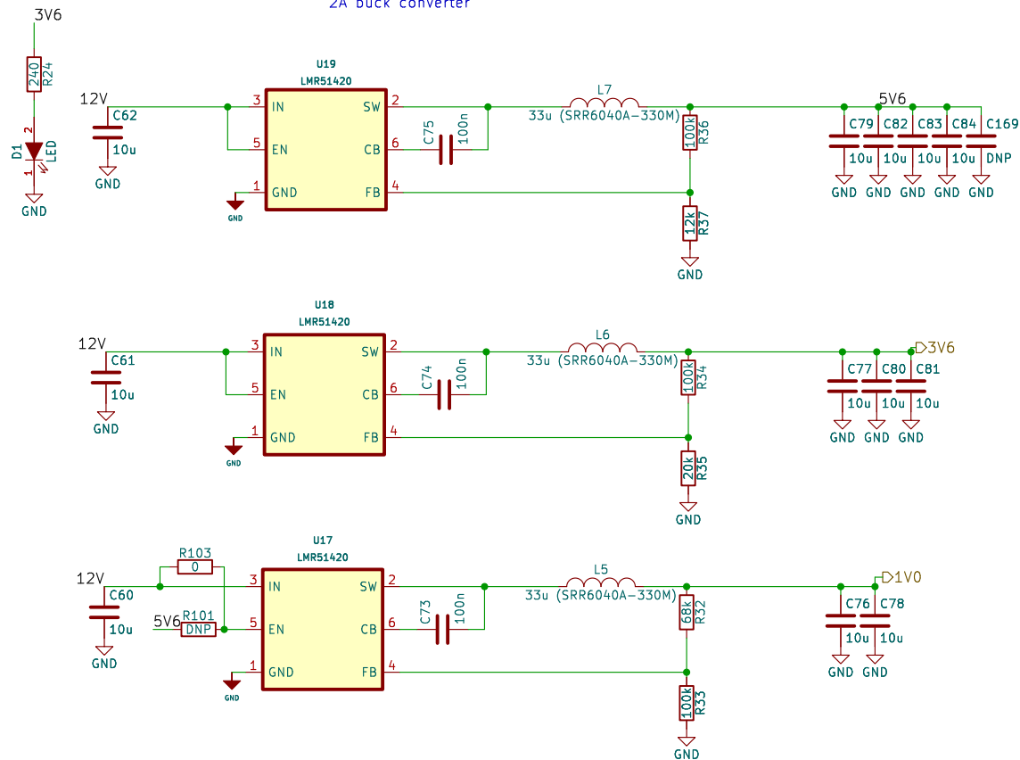
2A buck converter
