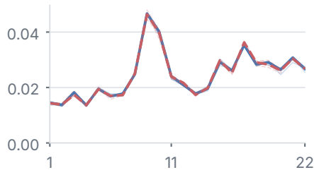
Classification / BERT
