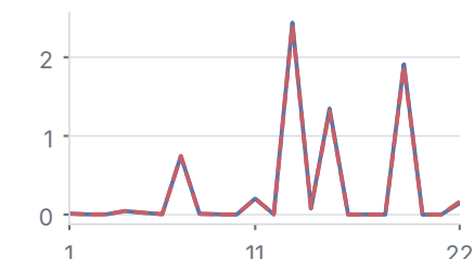
Video-text
