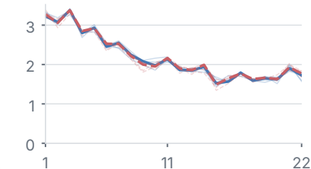
Process reward
