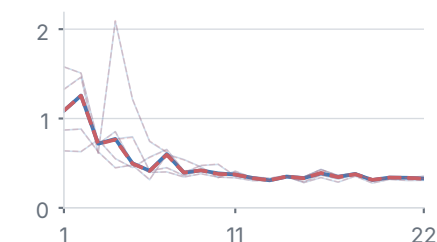
Video-text
