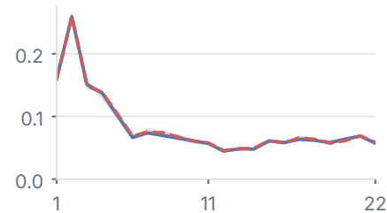
Cross-encoder
