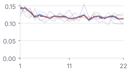
Classification / MPNet
