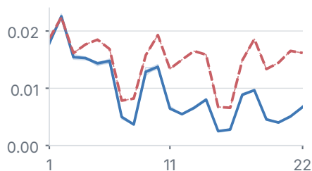
Outcome reward
