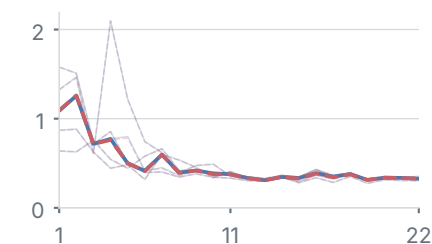
Video-text
