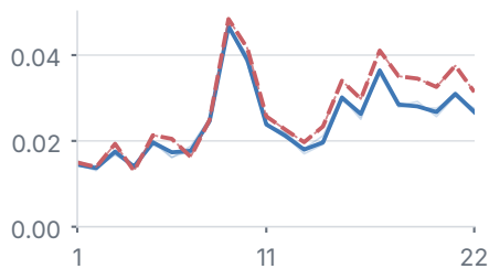
Classification / BERT
