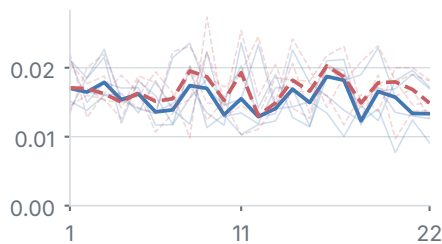
Classification / MPNet
