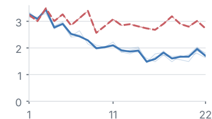
Process reward
