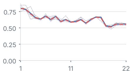
Audio-text
