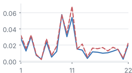
Image-text [C]
