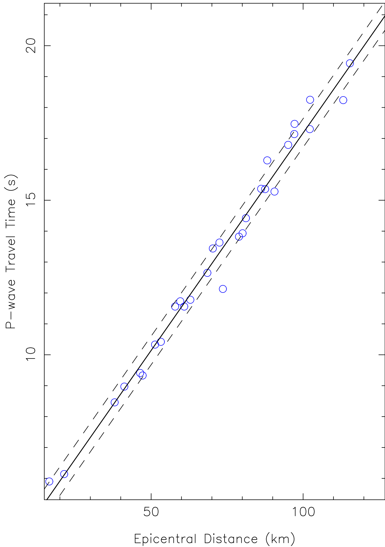
Linear Regression: P-wave Travel Time vs Epicentral Distance
