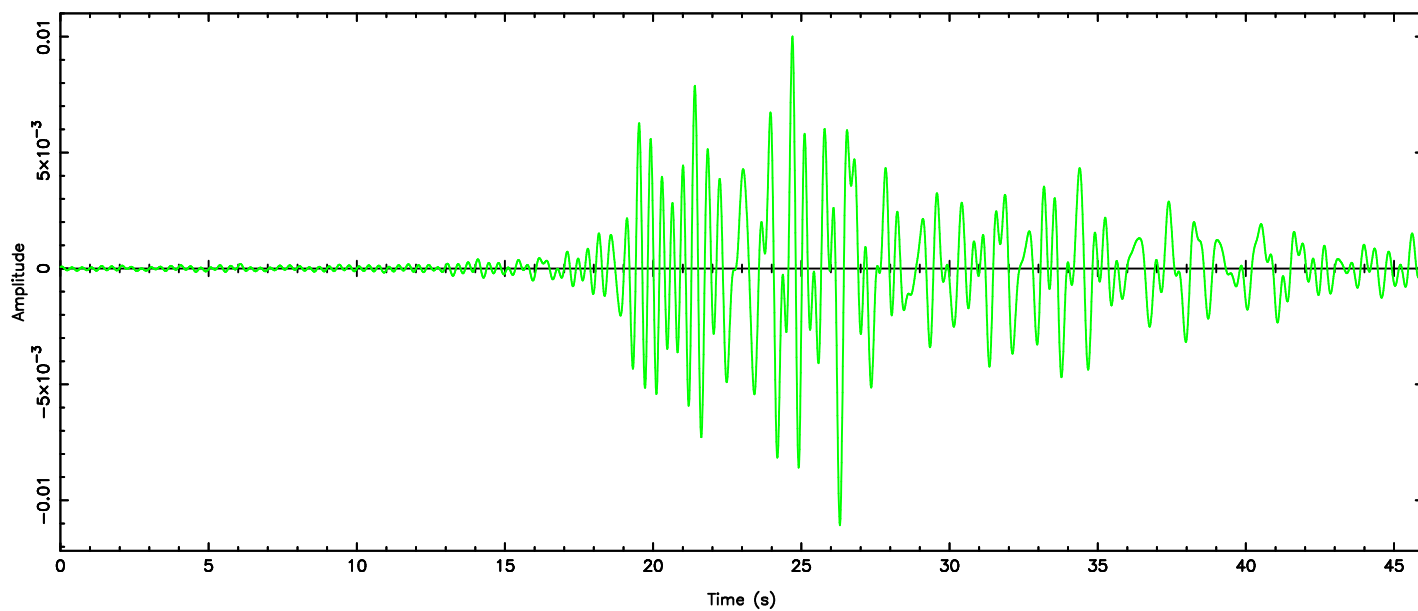
East–West Component (Filtered 0.5–3 Hz)
