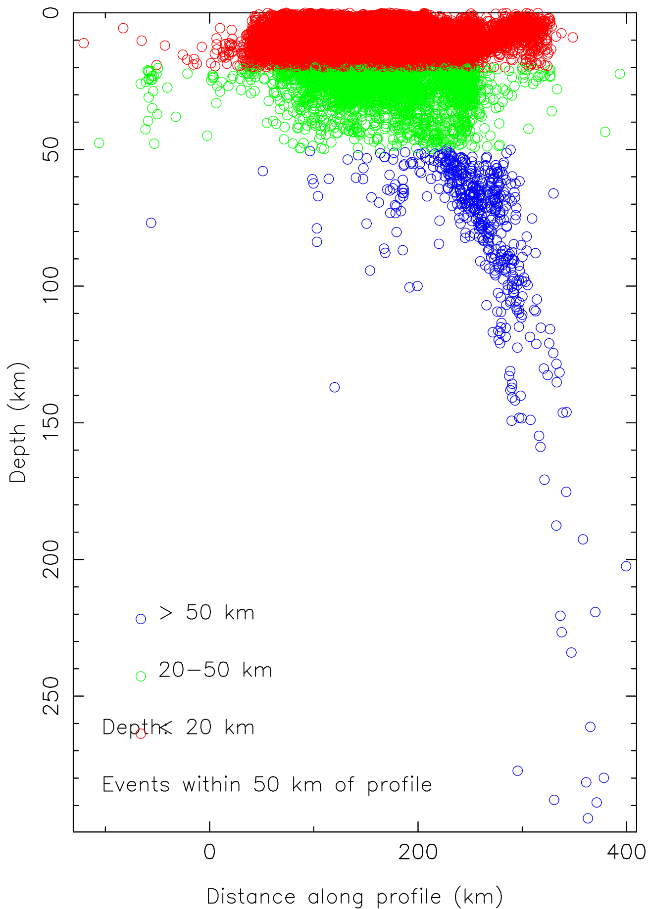
Earthquake Profile: (120., 23.) to (122., 25.0)
