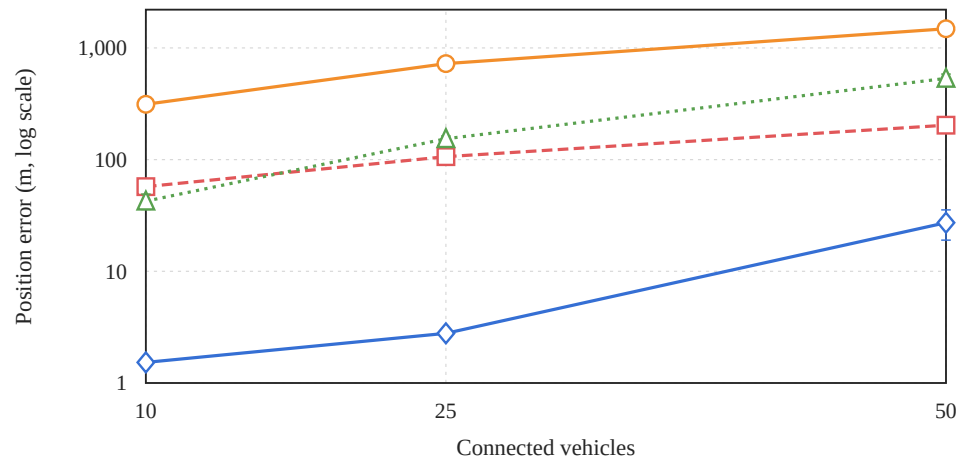
(b) DT synchronization error
