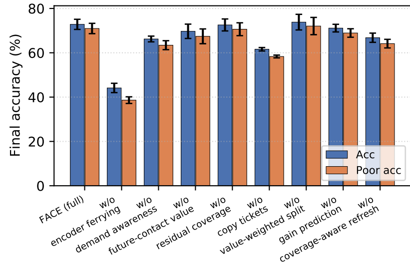
Uniform ECVs
