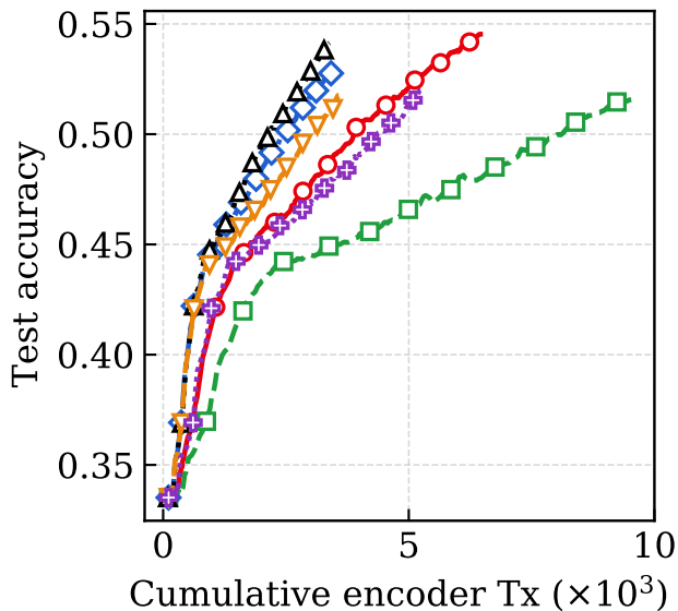
(a) KITTI
