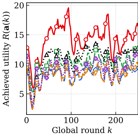
(a) KITTI
