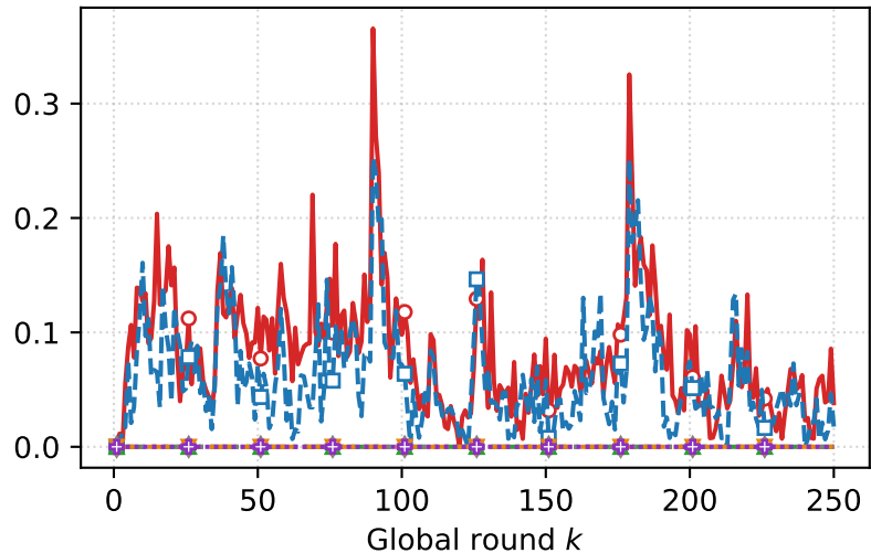
nuScenes
