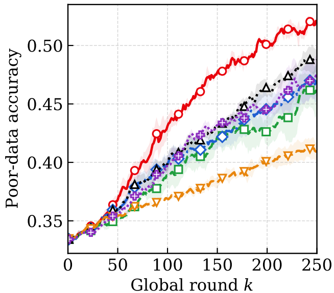
(a) KITTI
