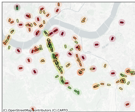
Learning-aware
