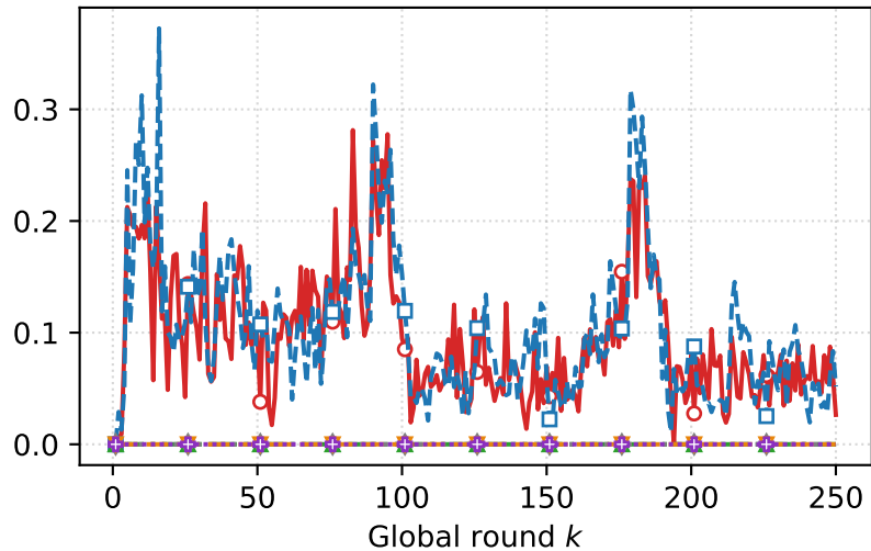
nuScenes
