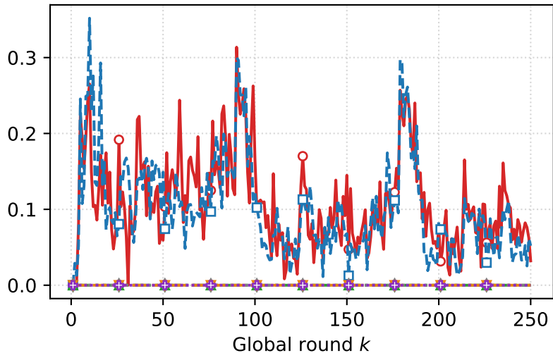
nuScenes
