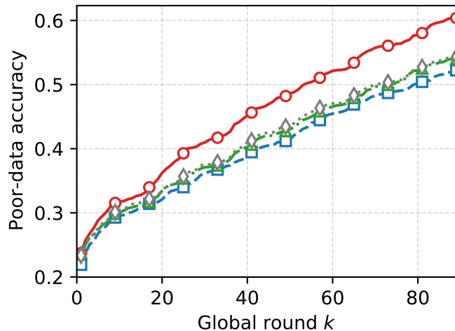
(b) Poor-data accuracy
