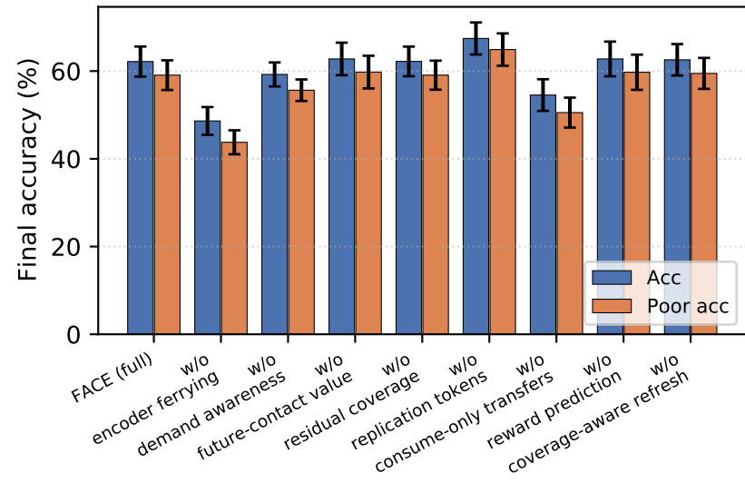
Uniform ECVs
