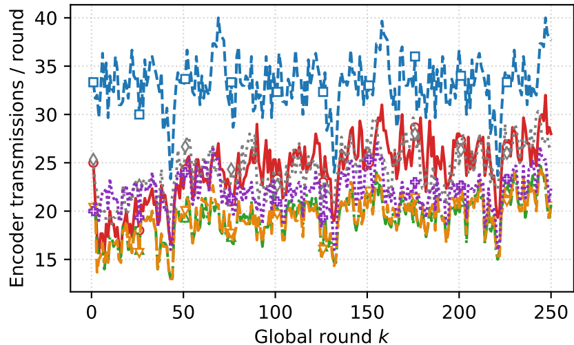
KITTI
