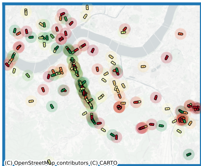
V2V-aware
