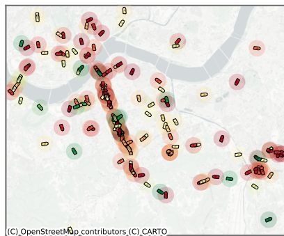
Learning-aware
