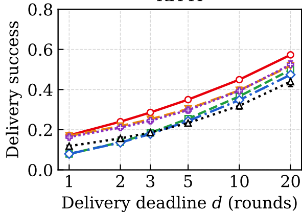
KITTI
