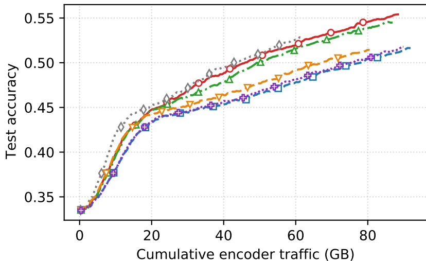
KITTI
