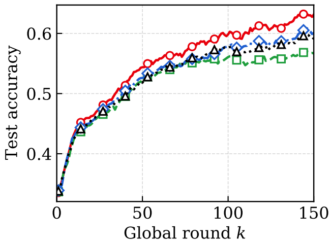
(c) KITTI
