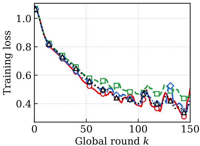
(a) KITTI
