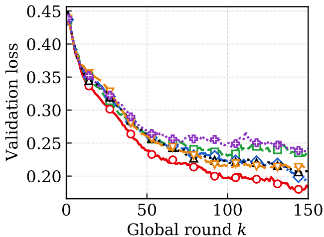
(a) KITTI
