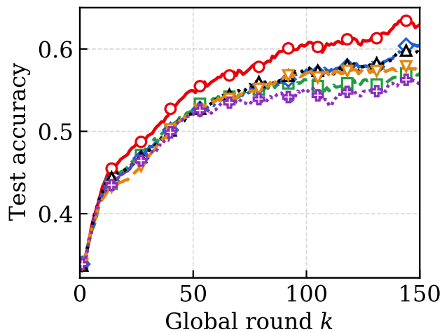
(c) KITTI
