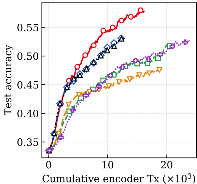
(a) KITTI
