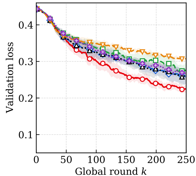
(a) KITTI
