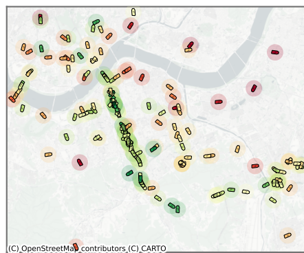
Learning-aware
