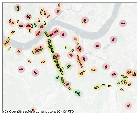
V2V-aware
