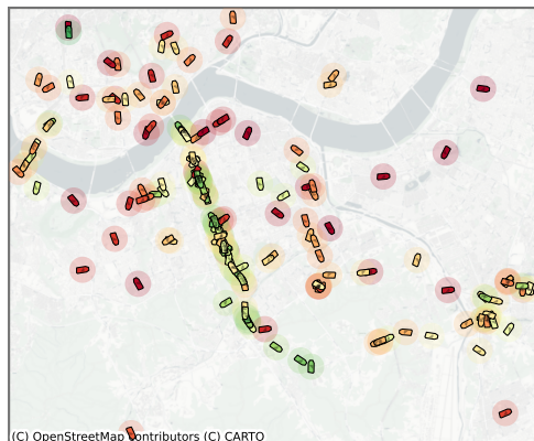
Learning-aware
