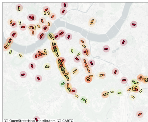
V2V-aware
