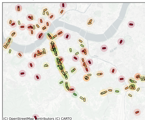
Learning-aware
