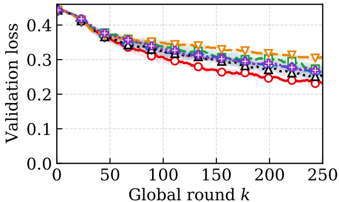
(a) KITTI
