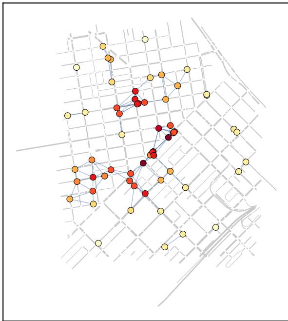
(a) SF downtown: 60 vehicles + V2V links
